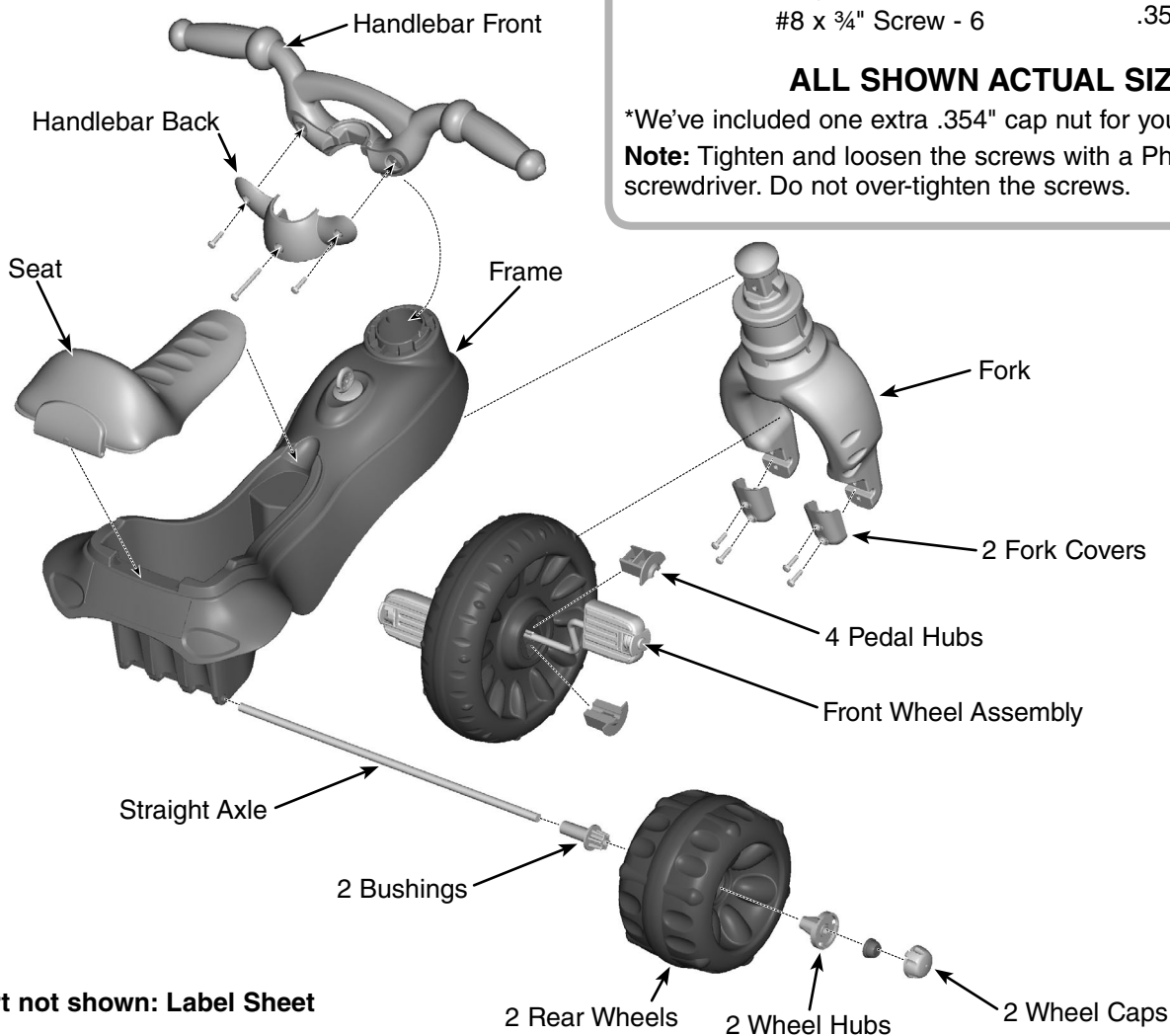
#8 x 3/4" Screw - 6
